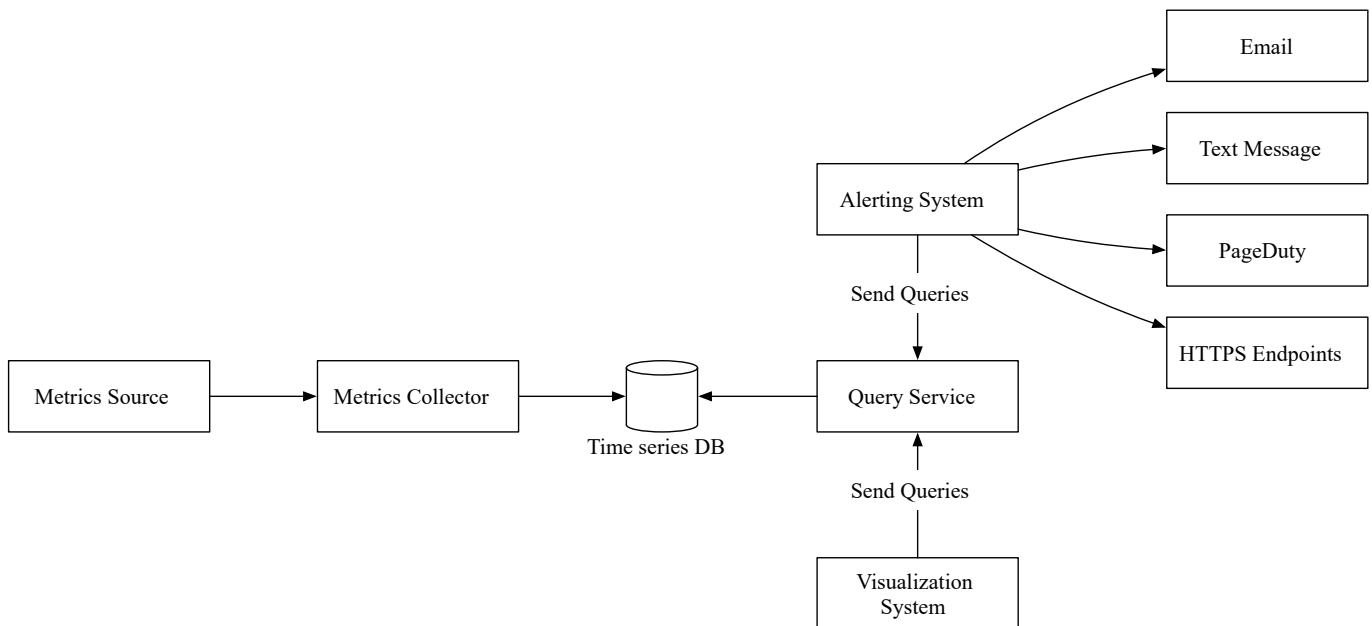
Figure 6 High-level design
