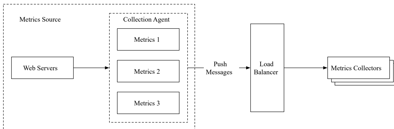
Figure 13 Load balancer
