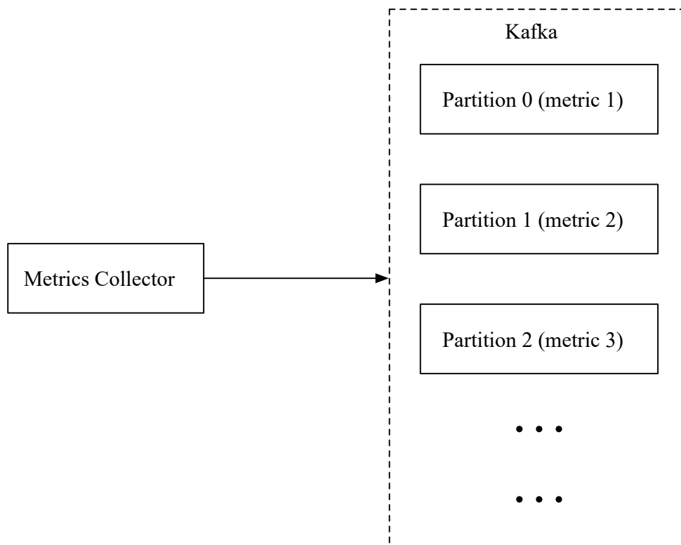
Figure 16 Kafka partition
