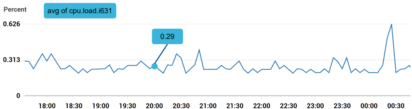
Figure 3 CPU load
